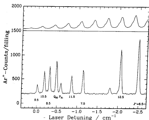
Fig. 3. Variation of the laser frequency in the region of the band head of the R_{11} branch of the N_2^+ [ A^2\Pi_u(v' = 2) \leftarrow X^2\Sigma_g(v'' = 0) ] transition. The temperature stabilized diode laser is tuned by scanning the injection current of the diode. Upper trace: Fringes of a 9.8 GHz etalon used for frequency calibration. Lower trace: Ar^+ ions from laser induced charge transfer are used as a monitor for detection of the spectrum.
