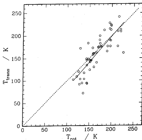
Fig. 6. Comparison of the translational and rotational temperature over a range from 100–250 K. The translational temperatures has been derived from the Doppler profile of the J'' = 7.5 line.
