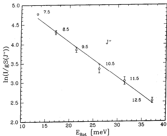
Fig. 4. Determination of the rotational temperature of \text{N}_2^+ from a Boltzmann plot. The logarithm of the measured intensities, which have been corrected for the laser power and divided by the nuclear spin multiplicities ( g ) and the Hönl–London factors S(J'') , are obviously close to a thermal population. The linear regression leads to a rotational temperature, T = (126 \pm 6) K that is in good agreement with the nominal temperature of the trap.
