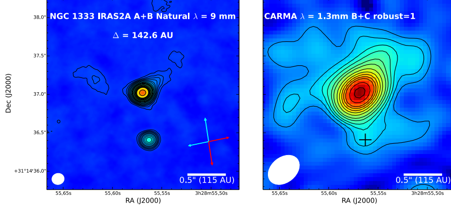
Figure 5: Maps of NGC 1333 IRAS 2A obtained with the JVLA at the wavelength of 9 mm (left) and with CARMA at the wavelength of 1.3 mm (right) (Tobin et al. 2015b). The higher angular resolution of JVLA observations, combined with the lower optical depth of the 9 mm emission, resolves two components of IRAS 2A that are separated by about 0.5'' . The rms noise values in the IRAS2A images are 5.4 \mu\text{Jy bm}^{-1} (9mm), and 1.5 \text{ mJy bm}^{-1} (1.3mm). Contours are plotted every 5\times the noise level.
