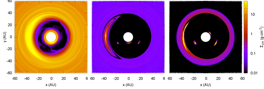
Figure 11: Snapshot of the gas and dust surface density of a disk perturbed by a 10 M_J planet orbiting at 20 AU from the central star, after 600 orbits of the planet. The planet is located at (0, -20) . Left: Gas surface density. A circular gap and a vortex develop at the orbital radius of the planet and at the outer edge of the gap, respectively. Center: Surface density of 1 mm grains. Millimeter grains are concentrated toward the center of the vortex (where the dust-to-gas ratio reaches values close to 1), and in the Lagrangian points on the planet orbit. Right: Surface density of 1 cm grains. Centimeter grains are even more concentrated toward the center of the vortex (modified from Fu et al., 2014).
