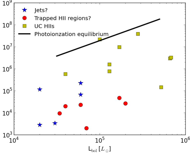
Figure 2: Ultracompact HII regions have radio fluxes close to the expectation from photoionization equilibrium and most likely are young, massive ( M_{\star} > 20 M_{\odot} ) stars with no further accretion. However, there is a population of fainter ionized sources that current facilities like the JVLA can only detect but cannot resolve. These sources could be small radio jets, stellar winds, or HII regions that are gravitationally trapped. Determining their nature is key for understanding the final stages of accretion in the formation of massive stars.
