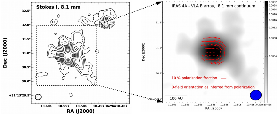
Figure 6: VLA B-config imaging of the deeply embedded protostar NGC 1333 IRAS 4A at 8.1 mm (37 GHz); Stokes I emission is shown in the left panel and the magnetic field orientations inferred from the polarized emission (rotated by 90^\circ ) are shown in the right panel. The grayscale in the right panel is the Stokes I emission. The rms noise is 23 \mu\text{Jy beam}^{-1} ; the contours start at 3\sigma and increase in intervals of \sqrt{2} . Credit: Erin Cox (Cox et al. 2015, submitted).
