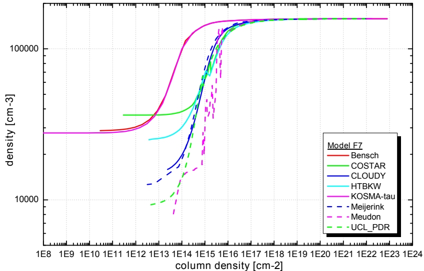
n(\text{H}_2) vs. N(\text{H}_2) - n=10^{5.5} \text{ cm}^{-3} , c=10^1 , variable T
