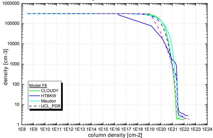
n(\text{H}) vs. N(\text{H}_2) - n=10^{5.5} \text{ cm}^{-3} , c=10^5 , variable T
